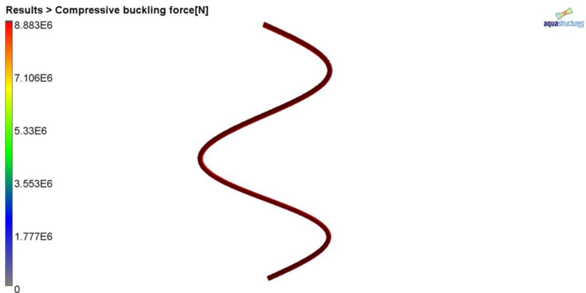
Figure 55 Calculation of buckling length and shape for a vertical beam with a node load on top
