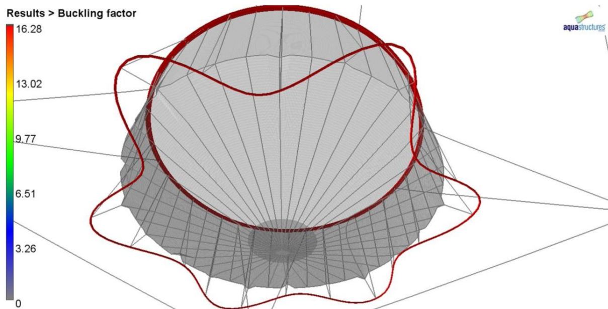
Figure 56 First buckling shape for a fish farm cage
