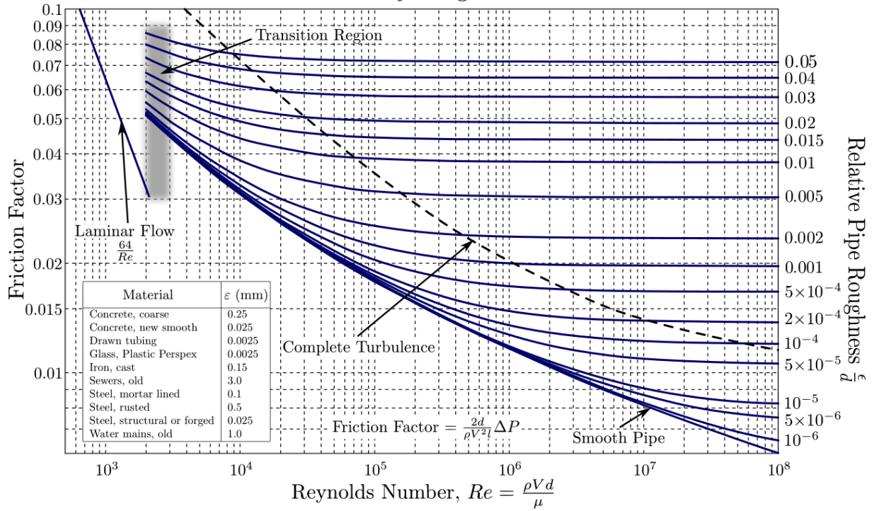
Figure 23 Moody chart (Wikipedia, 2020d)
