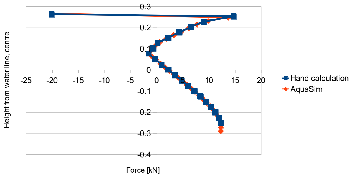
Figure 60 Comparison results, analytical formula and AquaSim analysis
