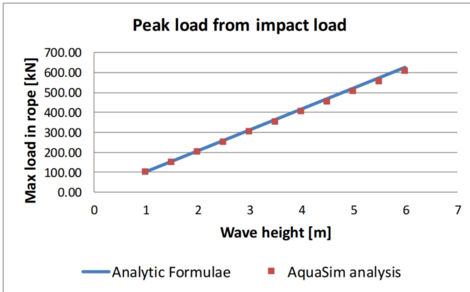
Figure 46 Response by analytical formulae to AquaSim analysis
