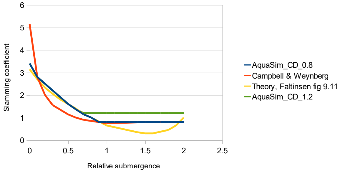
Figure 54 Comparison between AquaSim and Faltinsen and Campbell & Weynberg
