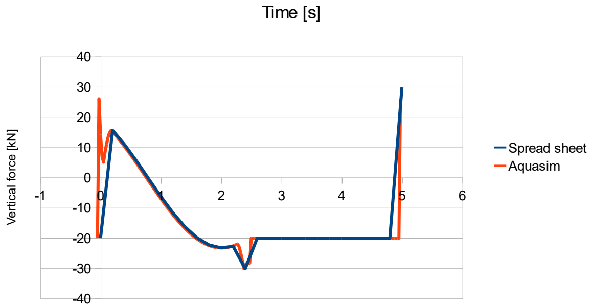
Figure 62 Comparison results, analytical formulae and AquaSim analysis
