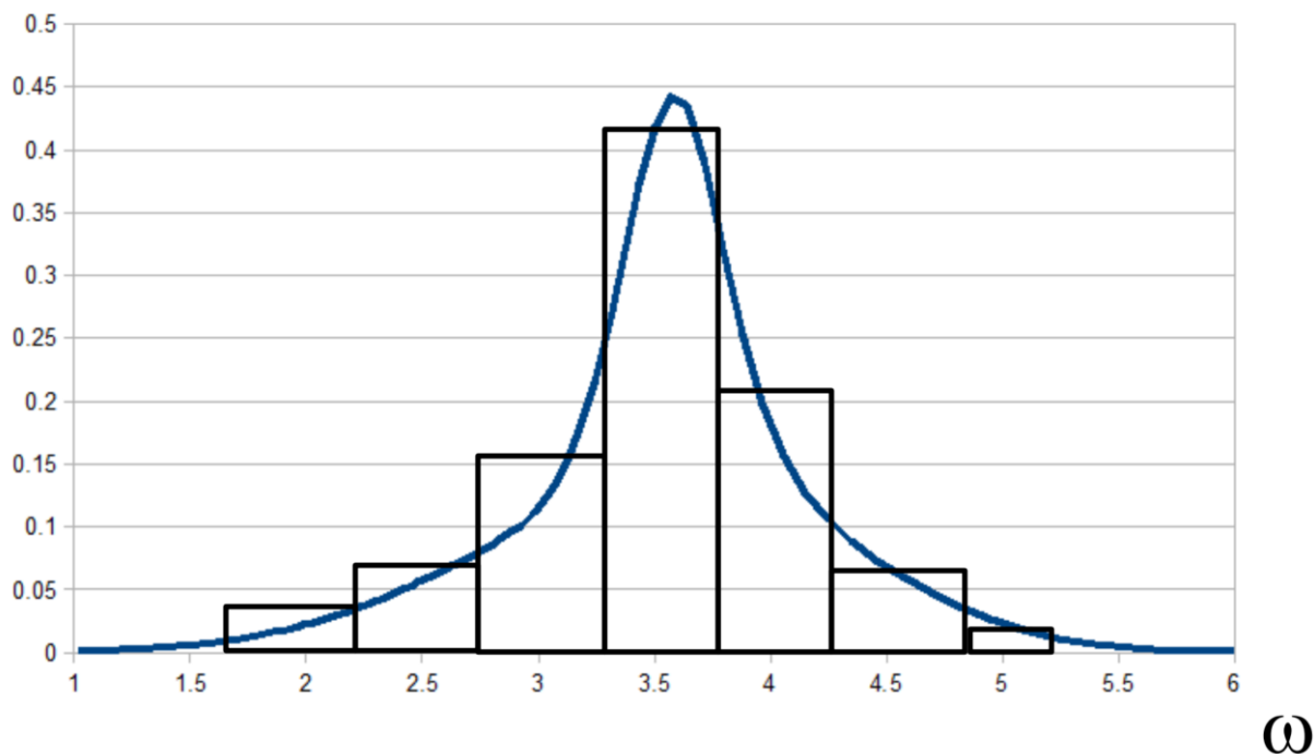
Figure 41 Discretization of wave spectrum
