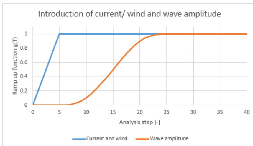
Figure 43 Introduction of current/ wind and wave amplitude as ramp up function vs. time step. Current is applied linearly over the initial steps (5 steps in this example). The dynamic part of the analysis uses 20 steps per wave period and a total of 40 time steps. Ramp up of wave amplitude is polynomial.
