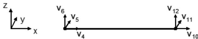
Figure 7 Truss element in a local coordinate system. Origin of local coordinate system is in node 1
