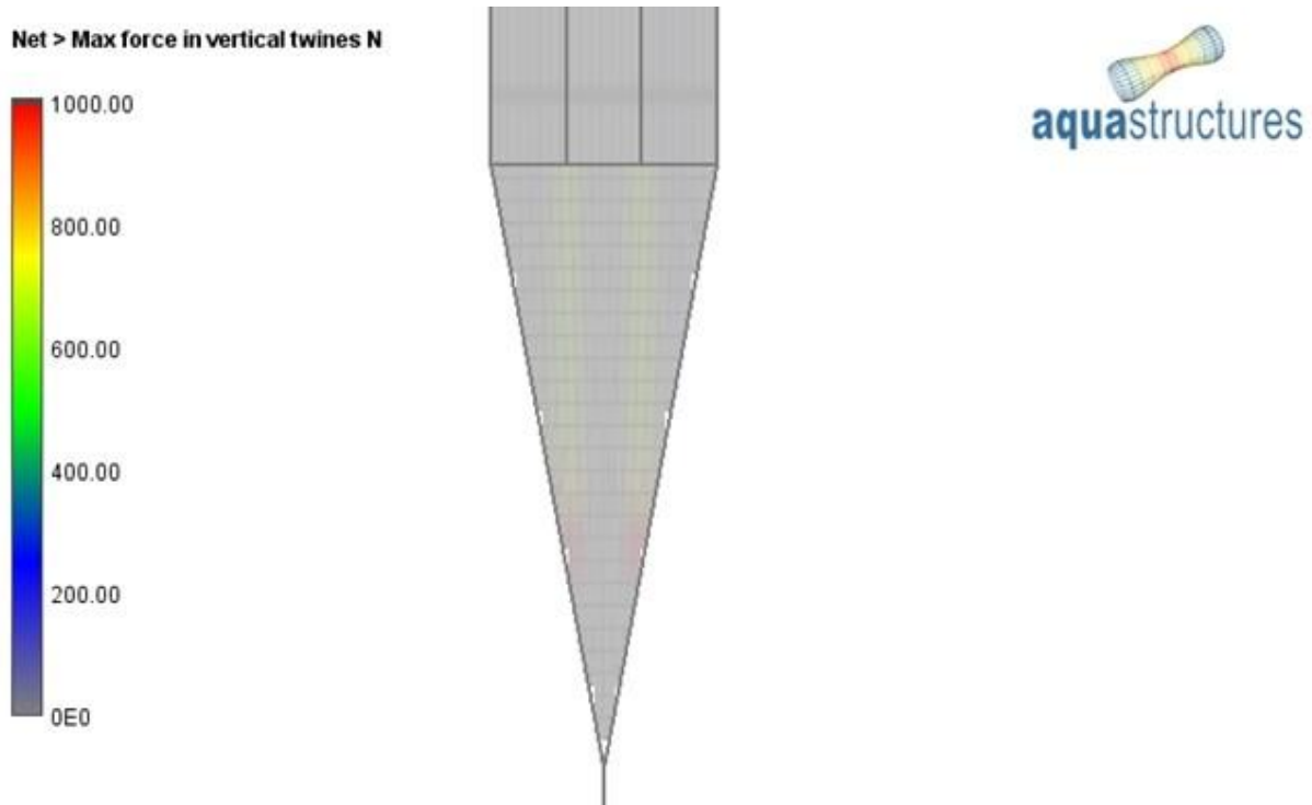
Figure 30 The conical part of the net modelled with parallel twines
