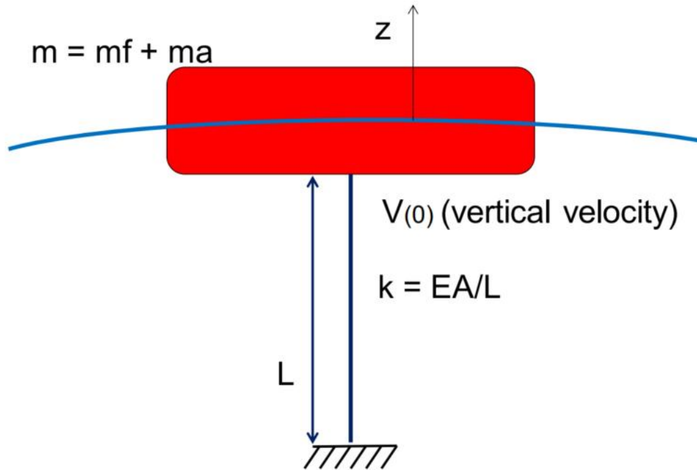
Figure 45 Initial value condition at moment rope goes stiff
