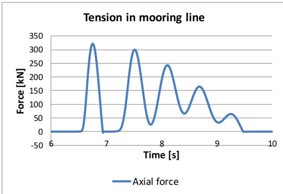
Figure 47 Tension in rope as a function of time
