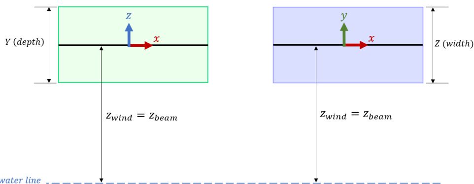
Figure 20 Average z -position applied in the calculation of wind velocity U
