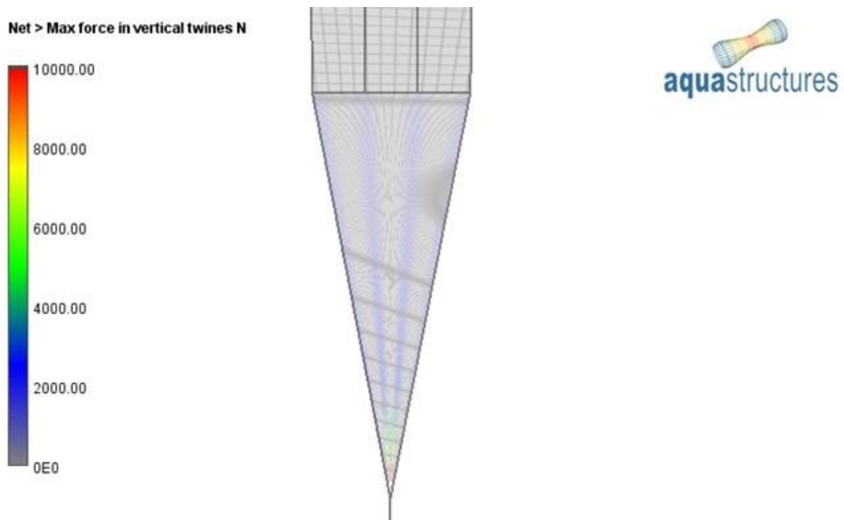
Figure 29 Forces in vertical twines, from AquaView
